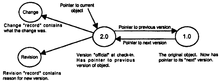
Figure 47 - Object Check-In
